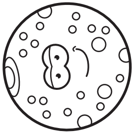
UMBRIEL
