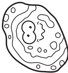
HYPERION
